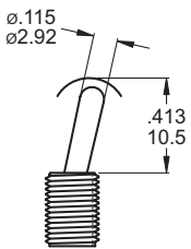
T6 FLATTED WITH ANTIROTATION
